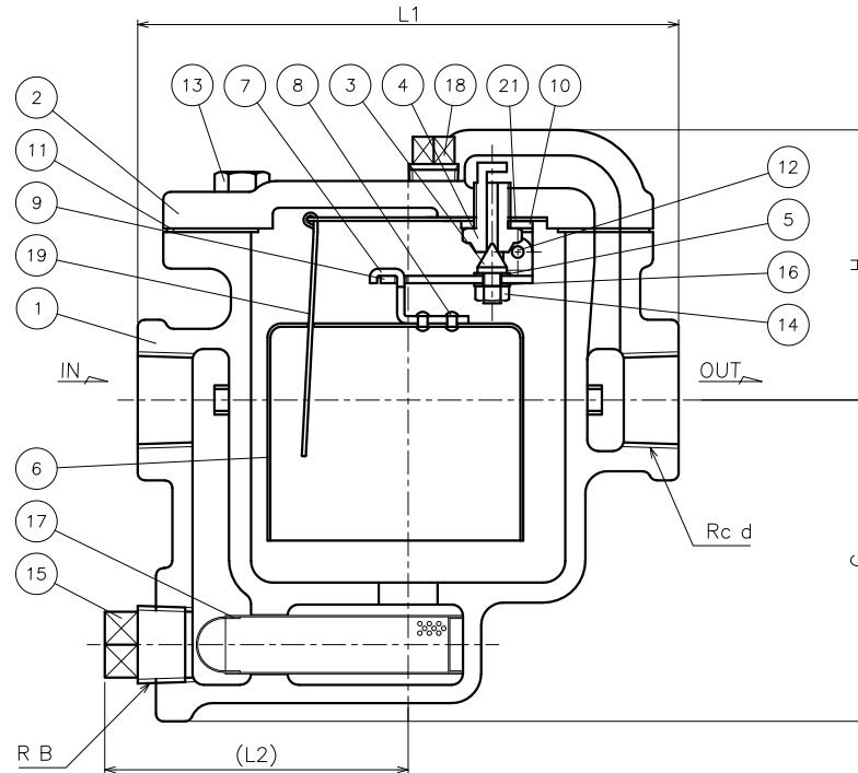
DIMENSIONS (mm)
