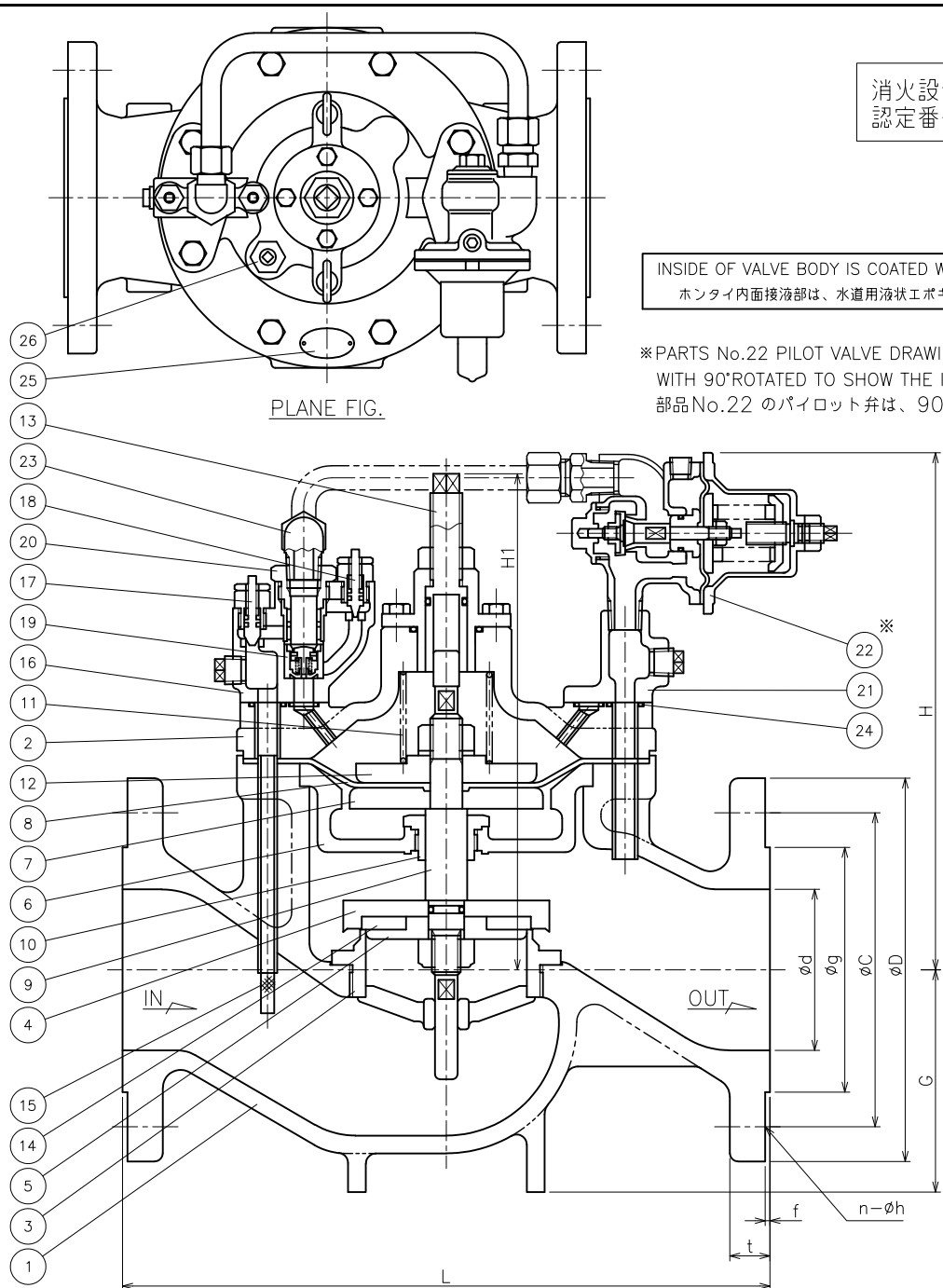
DIMENSIONS ( mm )
