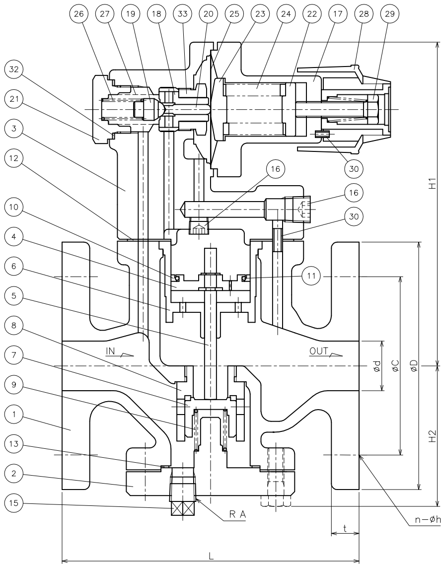
DIMENSIONS (mm) FLANGE CODE: JIS 10K
