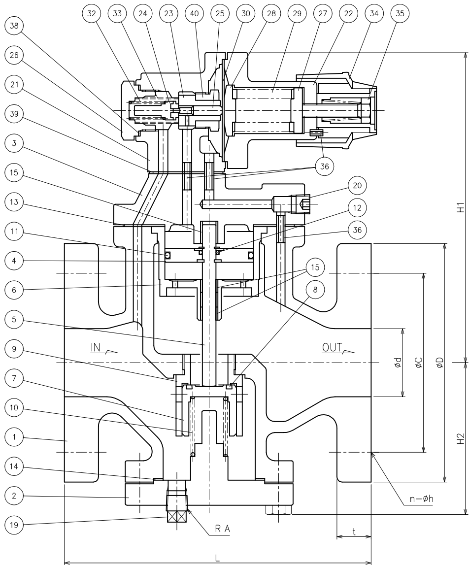
DIMENSIONS (mm) FLANGE CODE:JIS 10K
