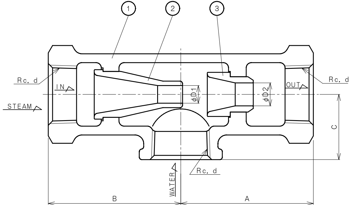
DIMENSIONS (mm)
