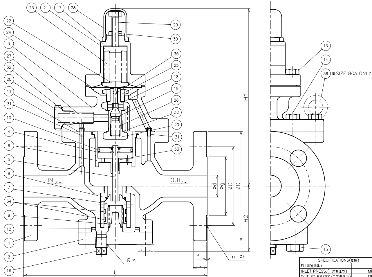
DIMENSIONS (mm)
