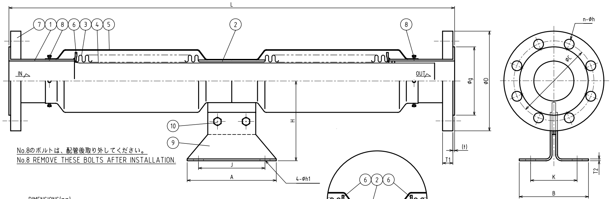
DIMENSIONS(mm)
