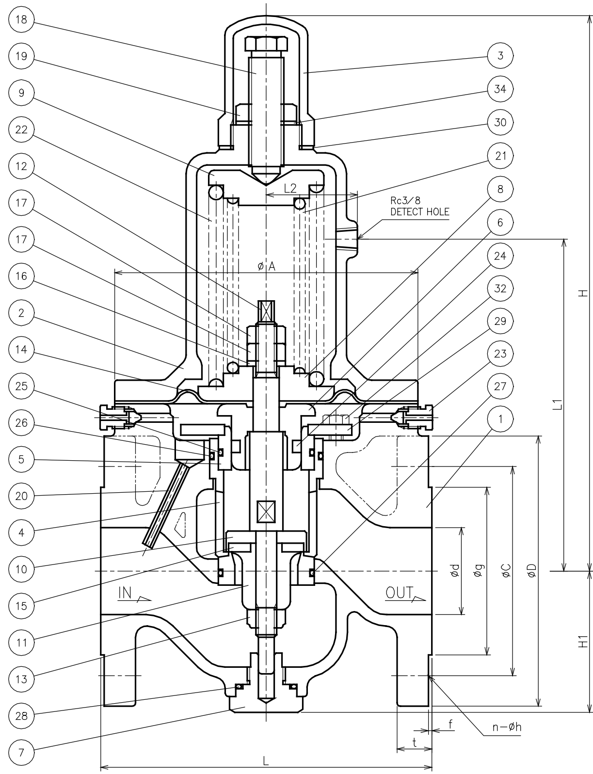
DIMENSIONS (mm) FLANGE CODE: JIS 10K
